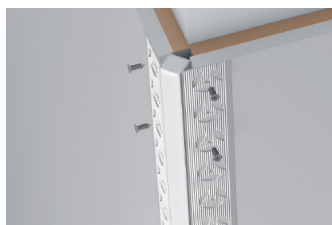
Fix the aluminum profile with screws
