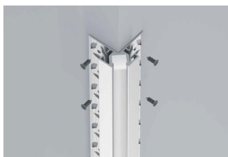
Fix the aluminum profile with screws
